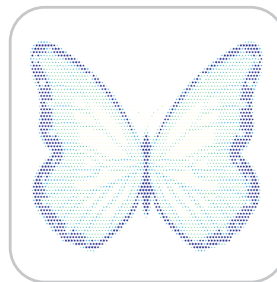
Rasterization
